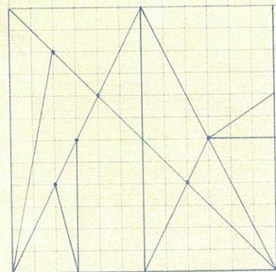
Archimedes: "Stomachion"
